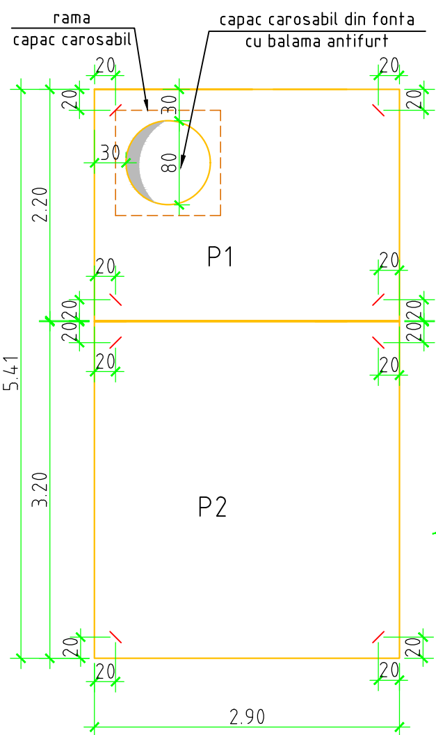
PLAN COFRAJ ANSAMBLU CAPAC PREFABRICAT
