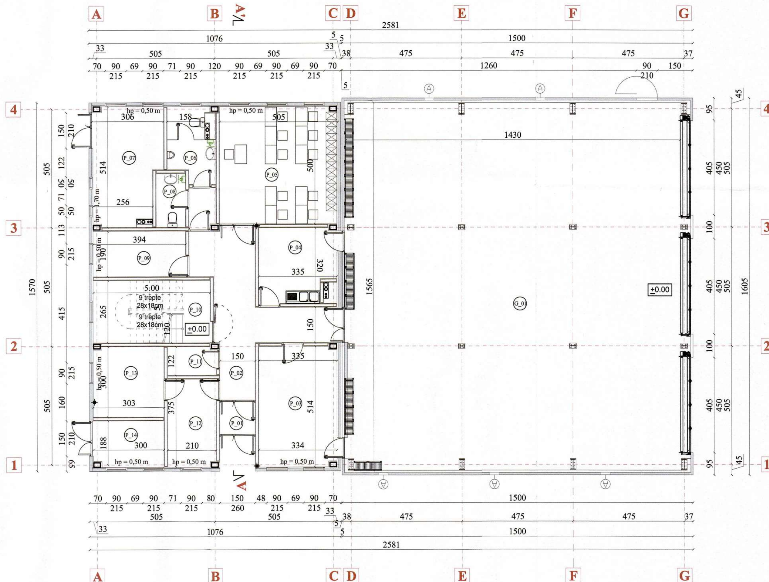
PLAN PARTER
